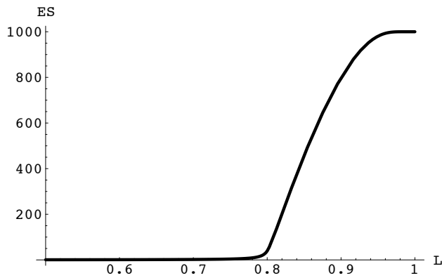
Figure 2: Mean number of components failed ES as a function of average initial component loading L . Note the change in gradient at the critical loading L = 0.8 . There are n = 1000 components and ES becomes 1000 at the highest loadings.
