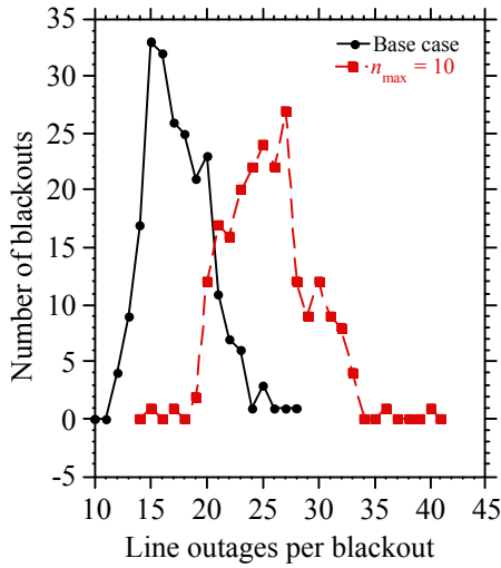
Figure 8. Distribution of the worst yearly blackouts for the base case and for n_{\max} = 10 .
