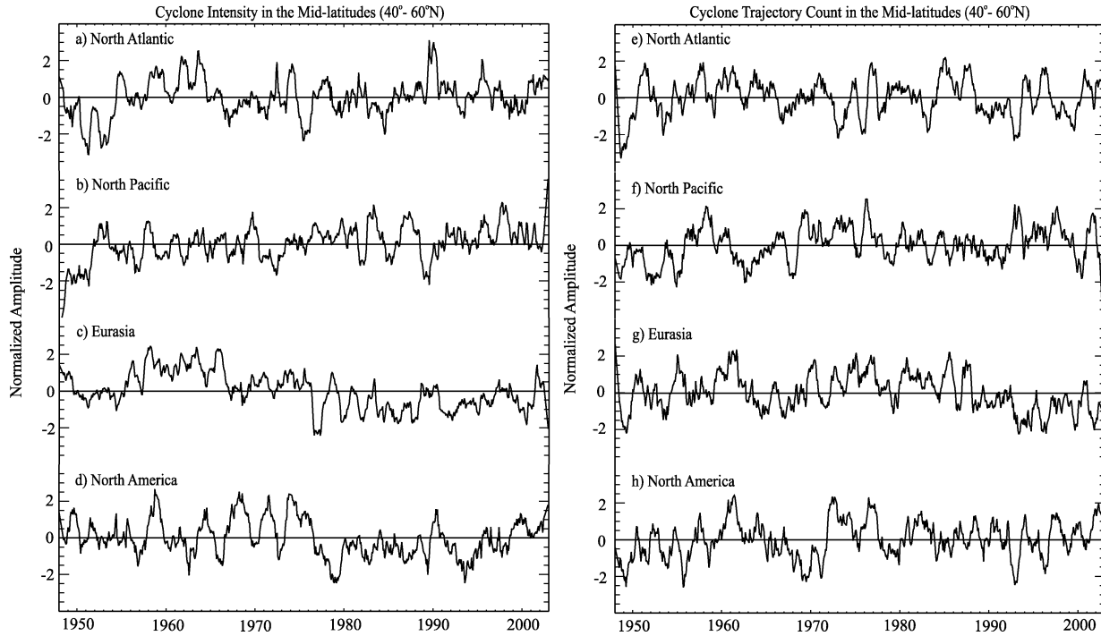
FIG. 10. The anomalies of cyclone intensity in (a) the North Atlantic, (b) the North Pacific, (c) Eurasia, and (d) North America. The anomalies of cyclone trajectory count in (e) the North Atlantic, (f) the North Pacific, (g) Eurasia, and (h) North America.
