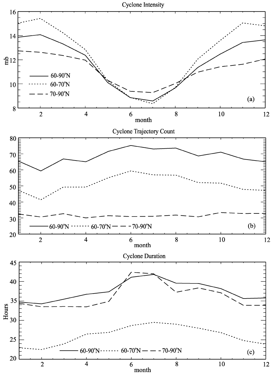
FIG. 3. The long-term mean seasonal cycle of cyclone (a) intensity, (b) trajectory count, and (c) duration in the Arctic region ( 60^{\circ} – 90^{\circ} N) and its two subregions, the Arctic Ocean ( 70^{\circ} – 90^{\circ} N) and the Arctic marginal zone ( 60^{\circ} – 70^{\circ} N). The units of intensity and duration are in hPa and h, respectively.
