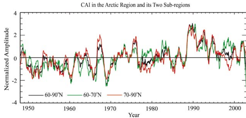
FIG. 5. The CAI anomalies for the Arctic region ( 60^{\circ} – 90^{\circ} N) and its two subregions, the Arctic Ocean ( 70^{\circ} – 90^{\circ} N) and the Arctic marginal zone ( 60^{\circ} – 70^{\circ} N), to which the 13-point smoother has been applied.
