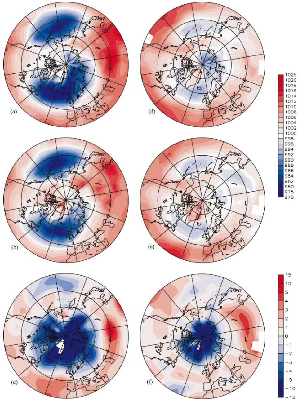
FIG. 14. The composite cyclone center SLP in the winters with the CAI anomalies (a) larger than 1.0 std dev, (b) less than -1.0 std dev, and (c) their difference. The composite cyclone center SLP in the summers with the CAI anomalies (d) larger than 1.0 std dev, (e) less than -1.0 std dev, and (f) their difference.
