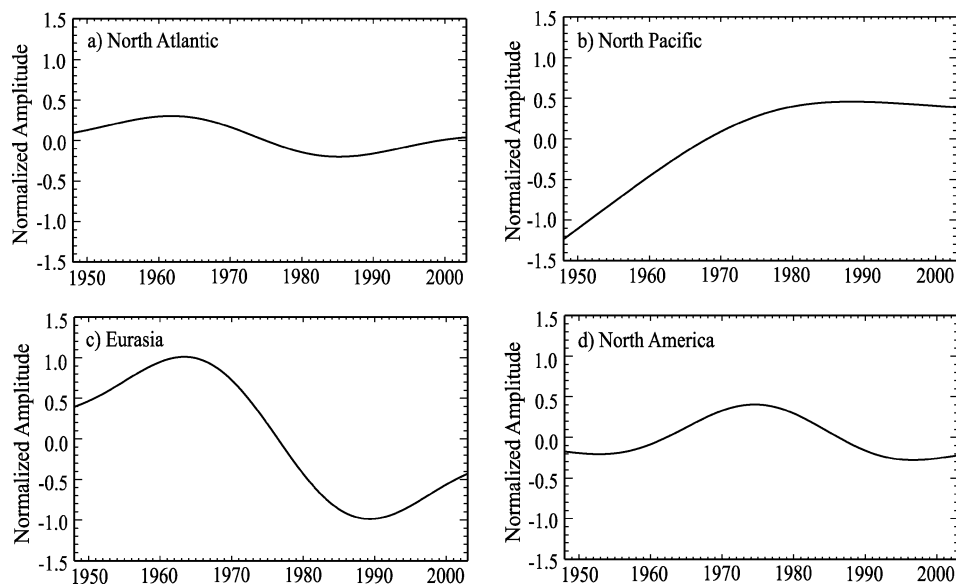
FIG. 8. The most significant low-frequency variation signals of CAI anomalies as determined by the MTM spectral analysis in the four midlatitude sectors: (a) the North Atlantic, (b) the North Pacific, (c) Eurasia, and (d) North America. The signals in (a)–(c) are significant at the 99% level and the signal in (d) is significant at the 95% level.
