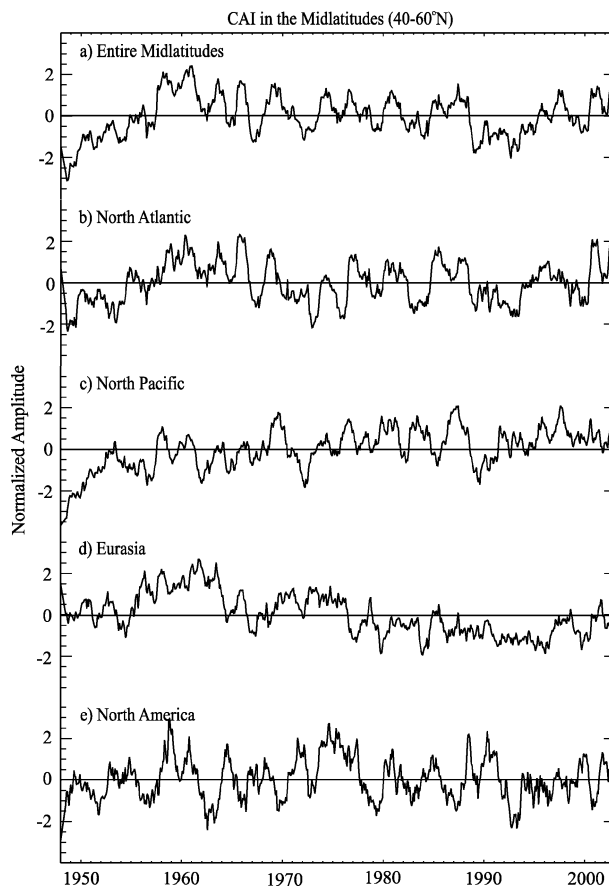
FIG. 7. The CAI anomalies in (a) the entire midlatitudes and its four sectors, (b) the North Atlantic, (c) the North Pacific, (d) Eurasia, and (e) North America.
