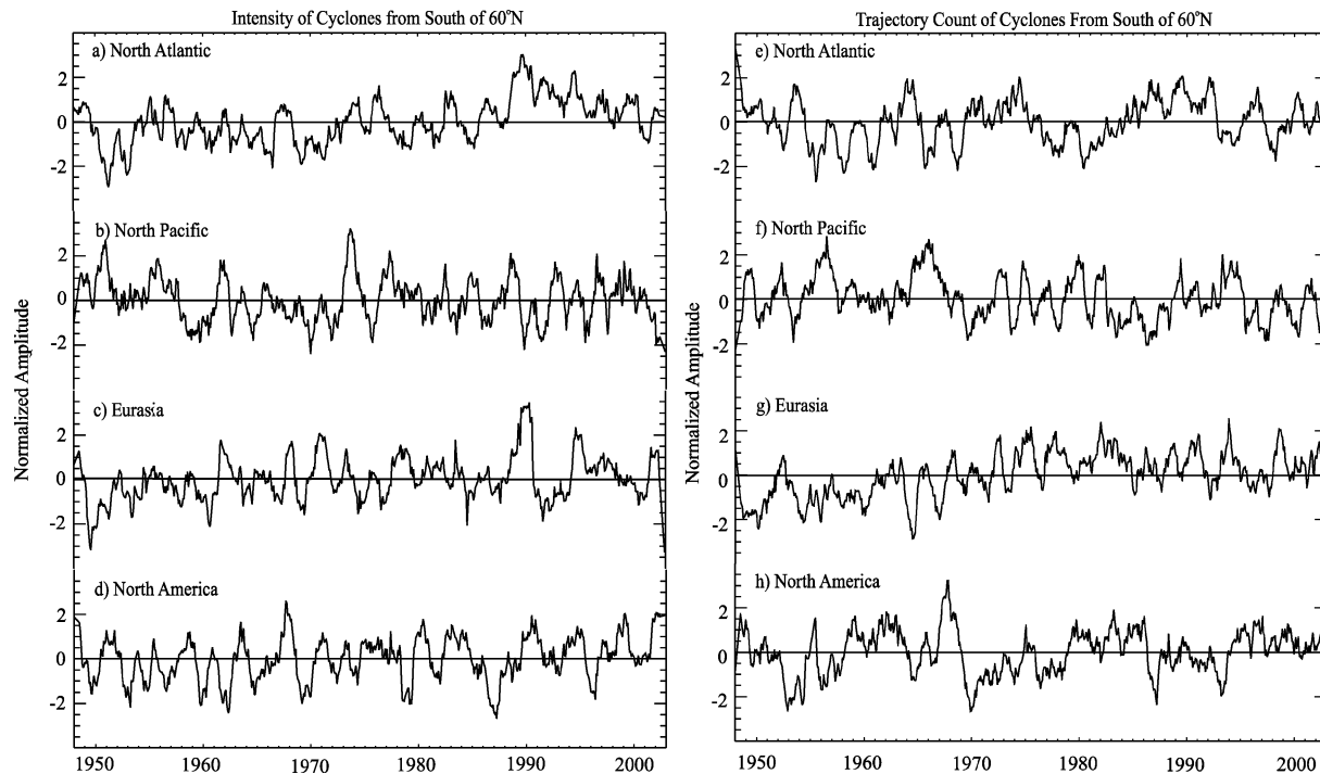
FIG. 12. The anomalies of cyclone intensity originating south of 60^{\circ} and passing through 60^{\circ}\text{N} in (a) the North Atlantic, (b) the North Pacific, (c) Eurasia, and (d) North America. The anomalies of cyclone trajectory count originating south of 60^{\circ} and passing through 60^{\circ}\text{N} in (e) the North Atlantic, (f) the North Pacific, (g) Eurasia, and (h) North America.
