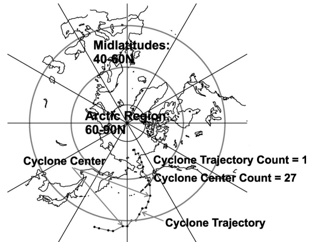
FIG. 1. A cyclone process from 0000 UTC 16 Dec to 1200 UTC 22 Dec 1999, which moves from 35.0^\circ\text{N} , 162.5^\circ\text{E} to 75.0^\circ\text{N} , 165.0^\circ\text{W} , schematically shows the difference of definitions between the cyclone trajectory count and the cyclone center count.
