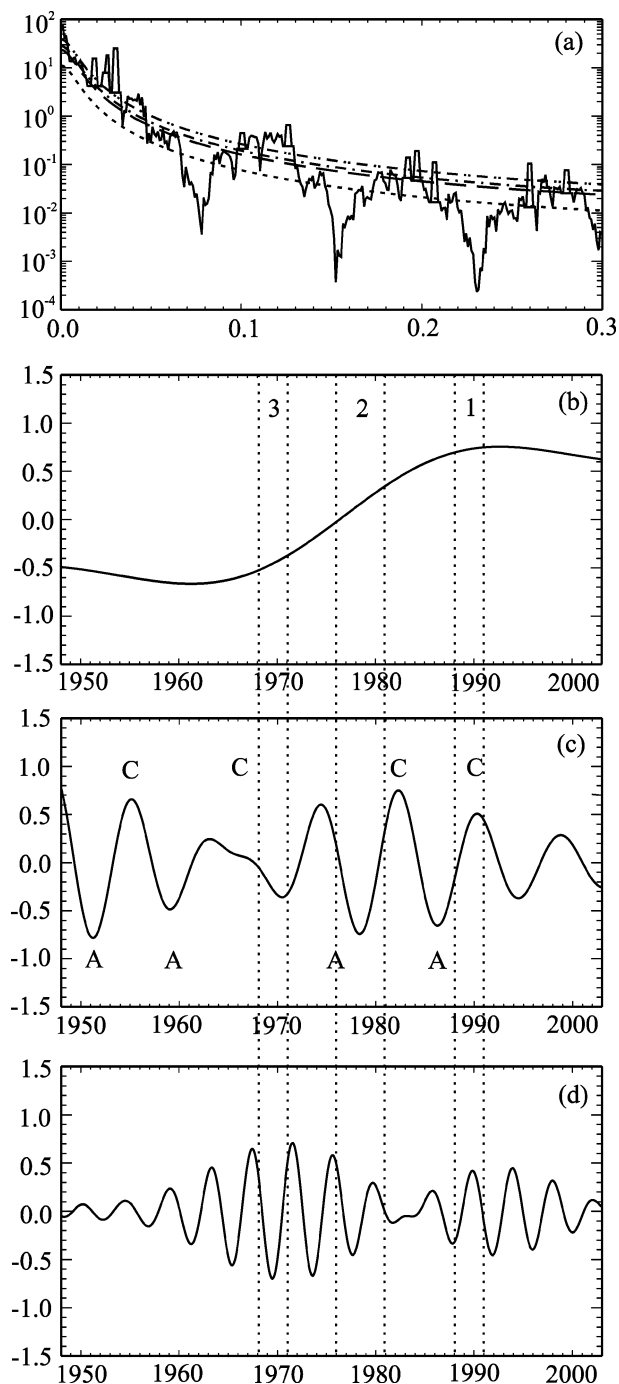
FIG. 6. (a) The MTM spectrum of the CAI anomaly time series for the entire Arctic region. The estimated red noise background and associated 90%, 95%, and 99% significant levels are shown by the short-dashed, the long-dashed, the dot-dashed and the double dot-dashed curves, respectively. The x coordinate is the frequency in cycles per month and the y coordinate is the spectrum. The bandwidth parameter p = 2 , and three tapers were used. (b)–(d) Reconstructed signals of the low-frequency variation and 7.8- and 4.1-yr oscillations. The numbers 1–3 in (b) represents three selected representative periods, which are bounded by the dashed lines from (b) to (d). The letters “C” and “A” represent the cyclonic and anticyclonic regimes of sea ice and ocean motion defined by Proshutinsky and Johnson (1997).
