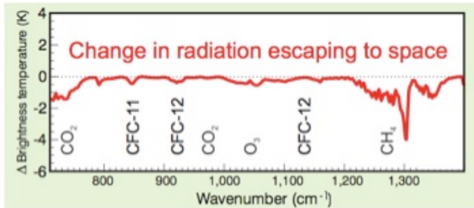
Figure 7.20: Change in the long-wave radiation released by Earth at the top of the atmosphere to space in 1997 compared to 1970. Absorption by water vapor, which overlaps with methane (CH 4 ), is between 1200 and 1400 cm -1 . Source of original graph is Harries et al., 2001; graph shown here is from Cook, 2010. Republished with permission of Nature Publishing Group/CCC and John Cook.
