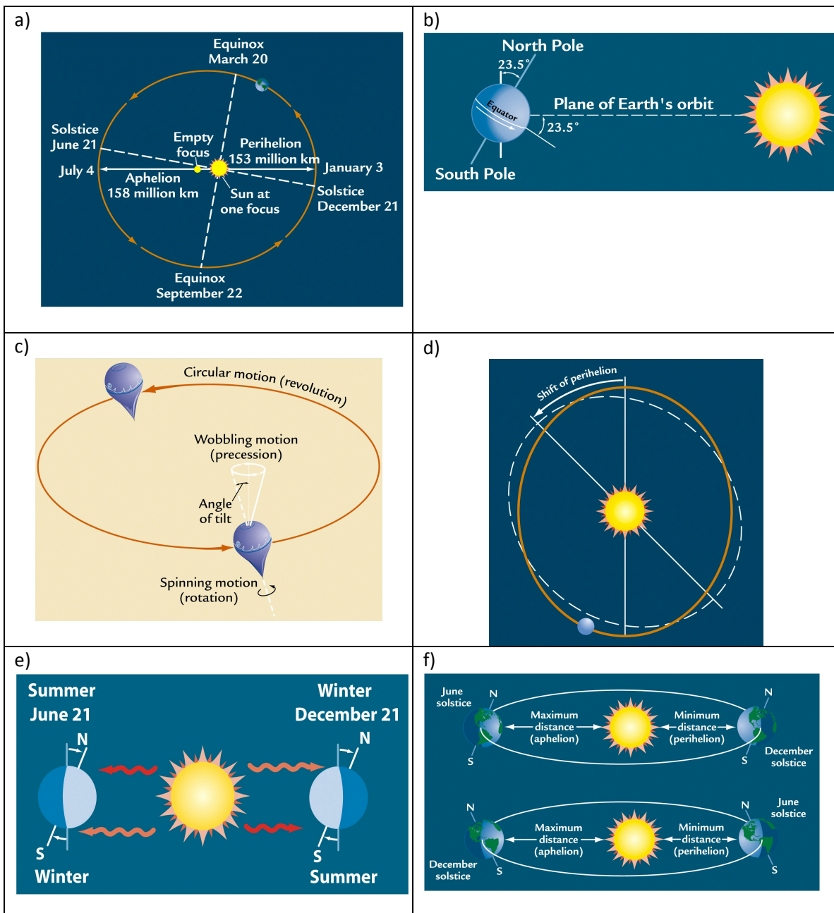
Figure 7.9: Summary of orbital factors that affect total solar radiation input to the Earth and its distribution by latitude. a) Elliptical orbit of the Earth around the Sun, with the Sun at one of the foci, b) Present day tilt of the Earth, c) Axial precession (wobbling motion), d) Precession of the equinoxes in space, e) Effect of tilt on the polar regions, and f) Extremes of the distance between the Earth and the Sun at the June and December solstices. Source: Ruddiman, 2008. Panels a, b, c, and e used with permission of W. H. Freeman and Son/Worth Publishers. Panel d adapted with permission of Woods Hole Oceanographic Institution/CCC. Panel f adapted with permission of American Association for the Advancement of Science/CCC.
