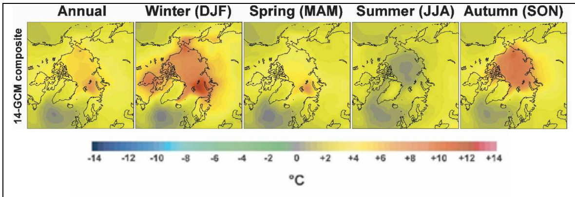
Figure 7.33: Arctic surface-air temperature change, relative to 1981–2000, for 2070–2089 based on the A1B greenhouse gas emissions scenario forecast by a composite of 14 global climate models. Source: Figure 13 from Chapman and Walsh, 2007. Used with permission of AMS/CCC.
