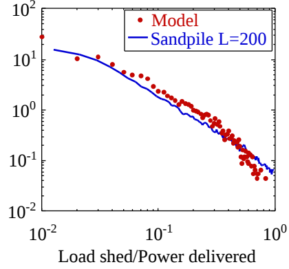
Fig. 10. PDF of the load shed divided by the power delivered compared to the PDF of the avalanches from a sandpile normalized to the maximum size.
