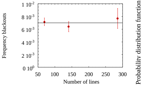
Fig. 9. Frequency of blackouts for the three tree networks listed in Table I.
