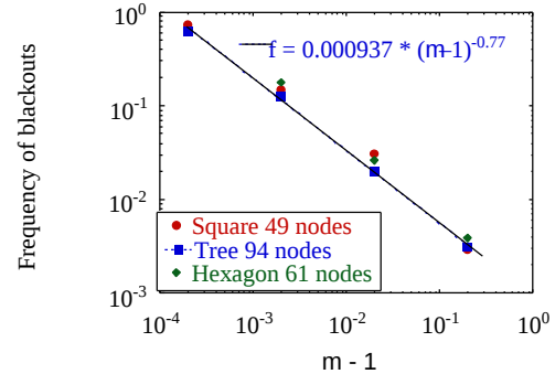
Fig. 5. Frequency of blackouts as a function of m for three different networks. The straight line is a power fit.
