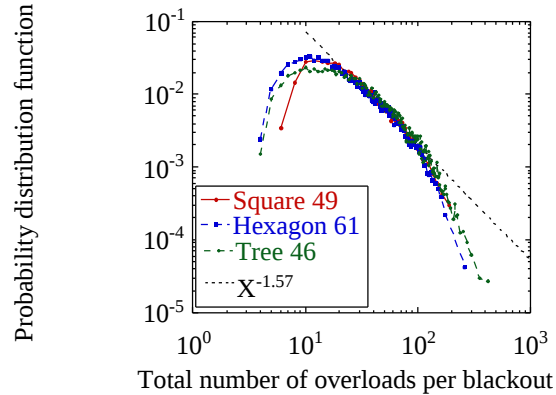
Fig. 8. PDF of the overloads for three different networks and for m=1.002 .
